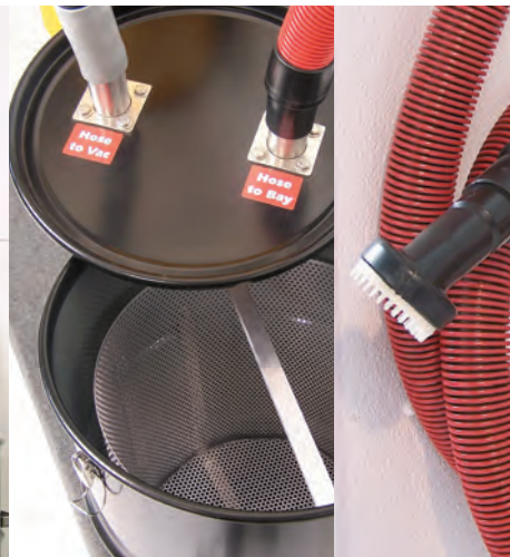
Detail of Clean Pet Vac Separator Tank and Grooming Nozzle
